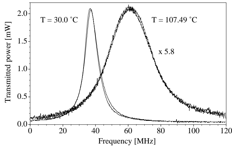
Figure 8.4: Lineshapes of the TEM_{00} resonator mode, 1064 nm input power was 125 mW. The phase matching for both curves is such that there nonlinearities do not cooperate. For T = 30.0^\circ\text{C} there is effectively zero nonlinear loss, the linewidth is due solely to mirror and cavity loss decay rates. For T = 107.49^\circ\text{C} the nonlinear loss is large, and the linewidth is accordingly broadened. No significant scanning asymmetries can be seen for either case: the thermal effect has been attenuated. The horizontal positions of the lineshapes are arbitrary.
