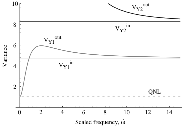
Figure 8.11: Theoretical Kerr squeezing spectra for Y_1, Y_2 quadratures. Scaled frequency, \hat{\omega} = \omega/\gamma_1 ; outcoupling, \hat{c} = 0.6 ; scaled detuning \hat{\Delta} = 15 ; scaled nonlinearity such that (\hat{\Delta} - \hat{n})(\hat{\Delta} - 3\hat{n}) = -3 ; and noisy pump V_{X_1}^{\text{in}1}(\omega) = 3, V_{X_2}^{\text{in}1}(\omega) = 10 observed at a quadrature angle \theta = \pi/6 . The squeezing is destroyed, but the output beam is still less noisy than the input beam on the Y_1 quadrature.
