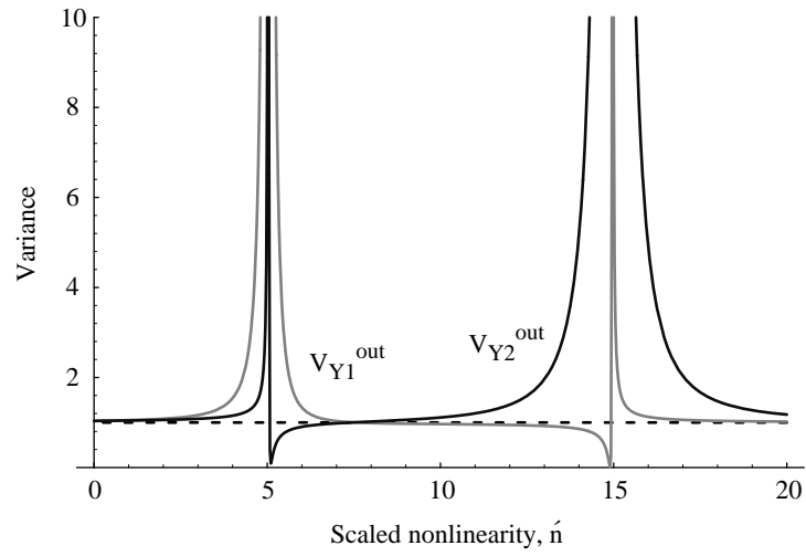
Figure 8.6: Y_1 & Y_2 quadratures versus scaled nonlinearity, \hat{n} = \mu|\alpha_1|^2/\gamma_1 . The pump is quantum noise limited V_{Y_1}^{\text{in}1}(\omega) = V_{Y_2}^{\text{in}1}(\omega) = 1 , the squeezing is observed at zero frequency, \omega = 0 for scaled detuning \hat{\Delta} = \Delta_1/\gamma_1 = 15 , and perfect outcoupling, \hat{c} = \gamma_1^c/\gamma_1 = 1 . Note that both quadratures are strongly squeezed, but at different nonlinearities.
