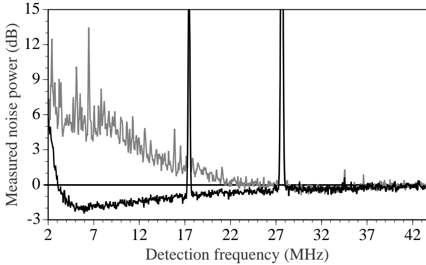
Figure 7.7: (a) Squeezing spectra. (a) Without competition, P_1 = 74 mW (b) With competition, P_1 = 60 mW.
