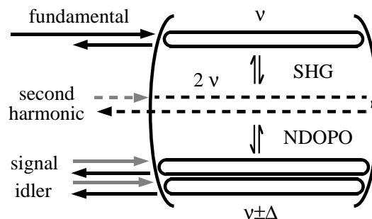
Figure 7.1: Conceptual layout of TROPO. Gray lines represent vacuum inputs, i.e. zero average power.
