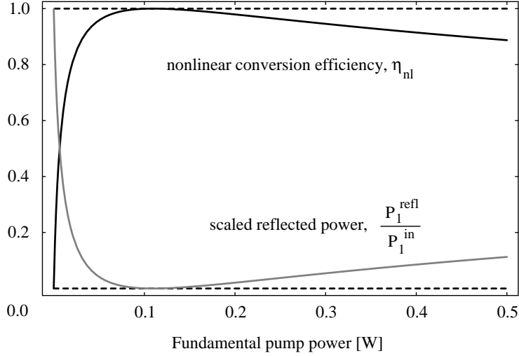
Figure 2.6: Nonlinear conversion efficiency, \eta_{\text{nl}} , and scaled reflected power, P_1^{\text{refl}}/P_1^{\text{in}} , versus incident power. Values used are: \mu = .002 ; R = 0.991 ; \gamma_1^c = \gamma_1 ; \tau = 1.863 \cdot 10^{-10} s; \lambda = 1064 nm.
